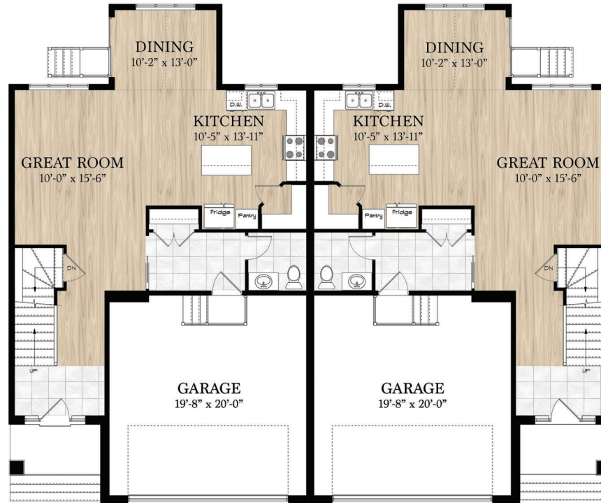
Main Floor Plan Living Area: 1753 sq. ft.
